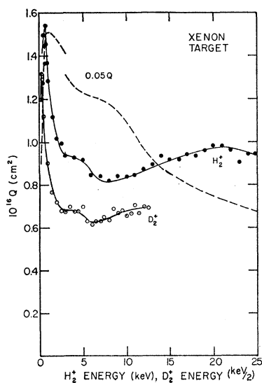
FIG. 3. Cross sections for Lyman-alpha production from H_2^+ and D_2^+ -Xe collisions. The dashed curve is the total charge-exchange cross section for H_2^+ +Xe from Stedeford and Hasted (footnote 7).
