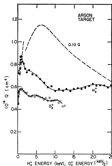
FIG. 4. Cross sections for Lyman-alpha production from H_2^+ and D_2^+ -Ar collisions. The dashed curve is the total charge-exchange cross section for H_2^+ +Ar from Stedeford and Hasted (footnote 7).
