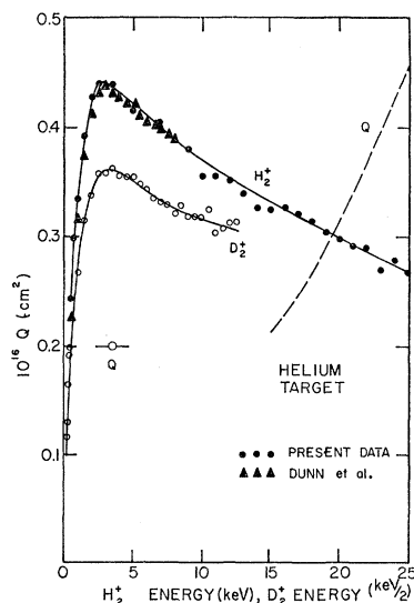
FIG. 1. Cross sections for Lyman-alpha production from H_2^+ - and D_2^+ -He collisions. The dashed curve is the total charge-exchange cross section for H_2^+ on He from Stedeford and Hasted (footnote 7). Present results are normalized to the data of Dunn et al. (footnote 2) at 6-keV H_2^+ energy.
